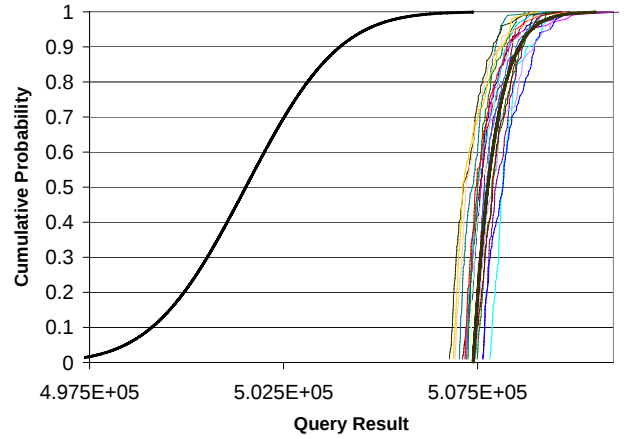
Figure 5: Observed empirical CDFs versus analytic CDF
