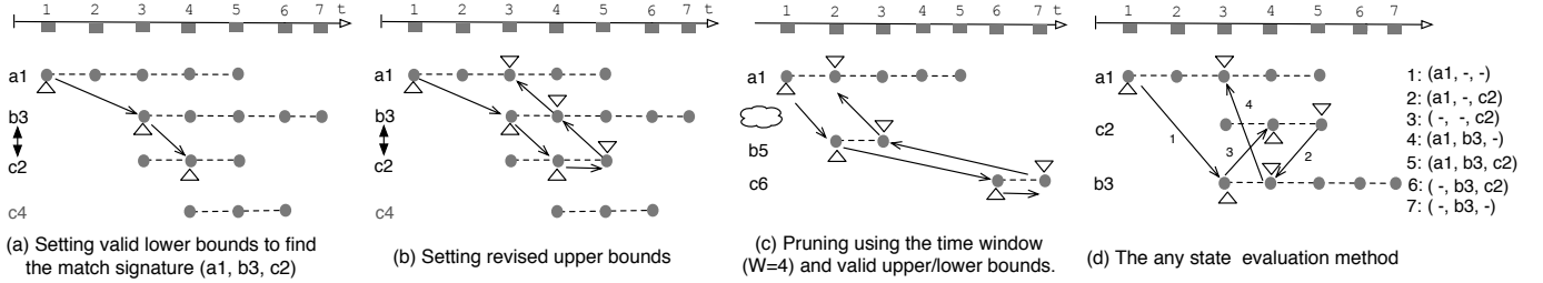
Figure 3: Illustration of the event-based evaluation (assuming that events are presented in query order).
